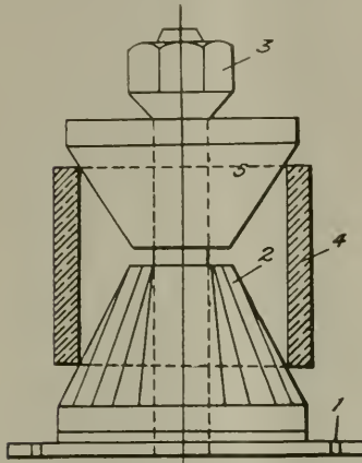
SPECIAL CHUCK FOR TURNING OF SIDE RODS
